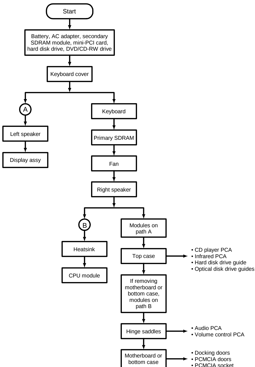
Figure 2-1. Disassembly Flow
