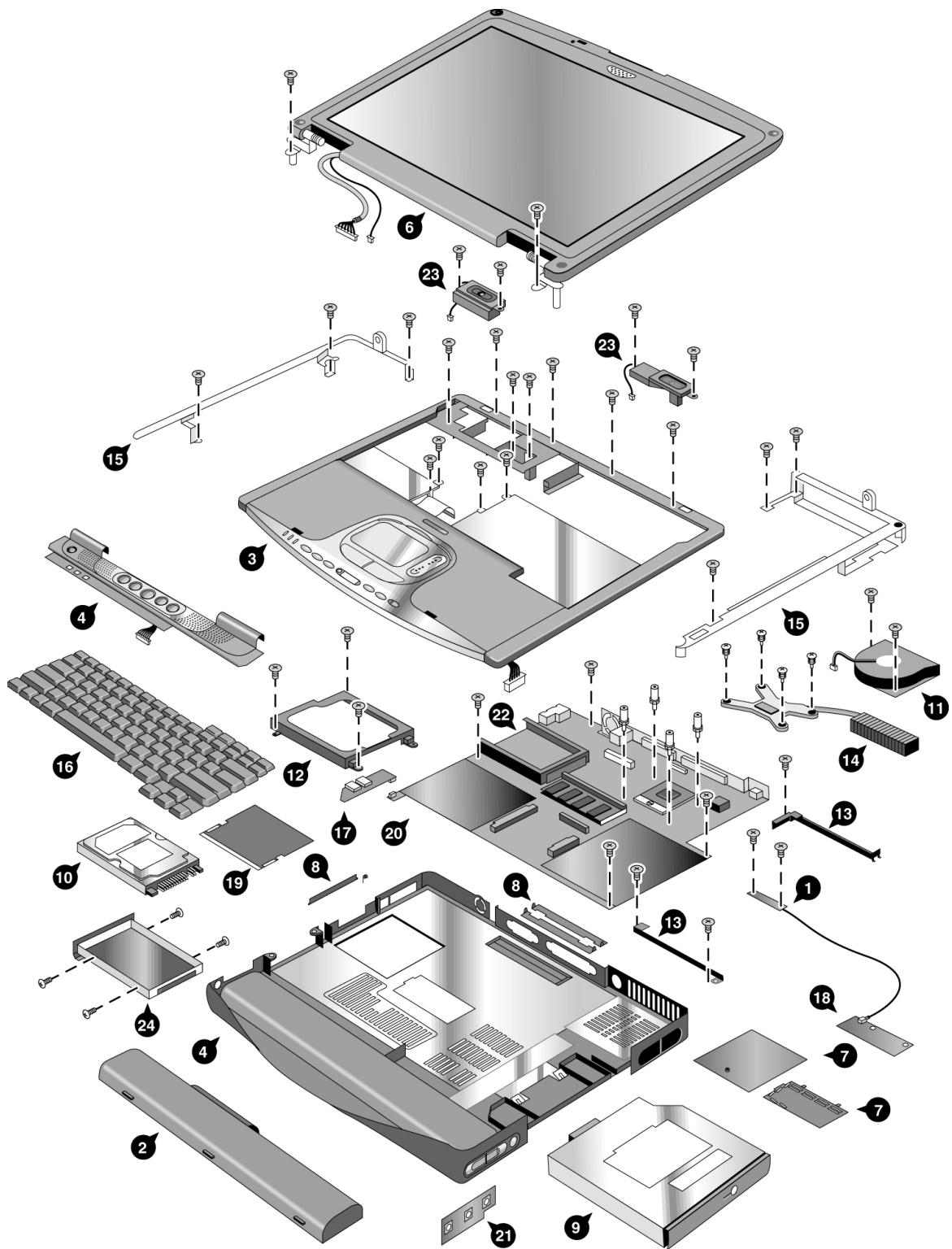
Figure 4-1. Exploded View
