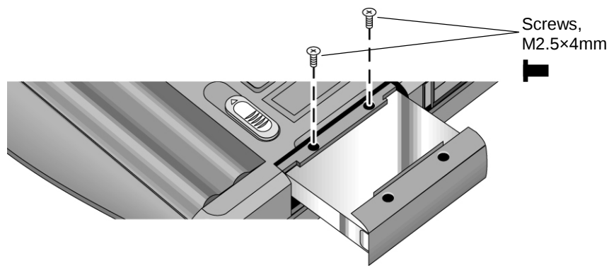
Figure 2-4. Removing the Hard Disk Drive
