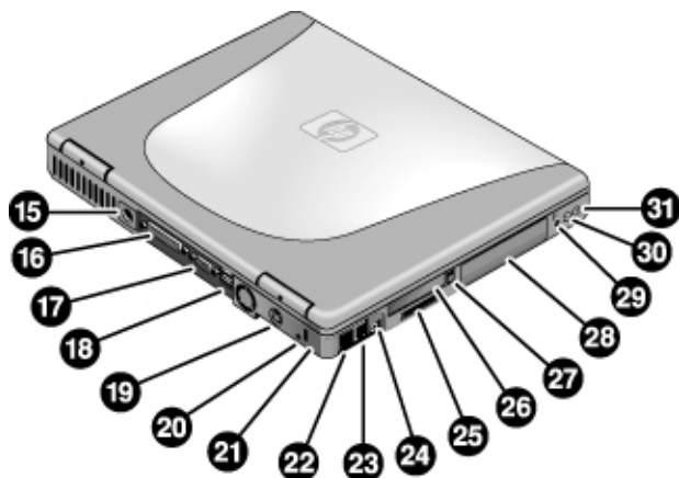
Figure 1-2. Back View
